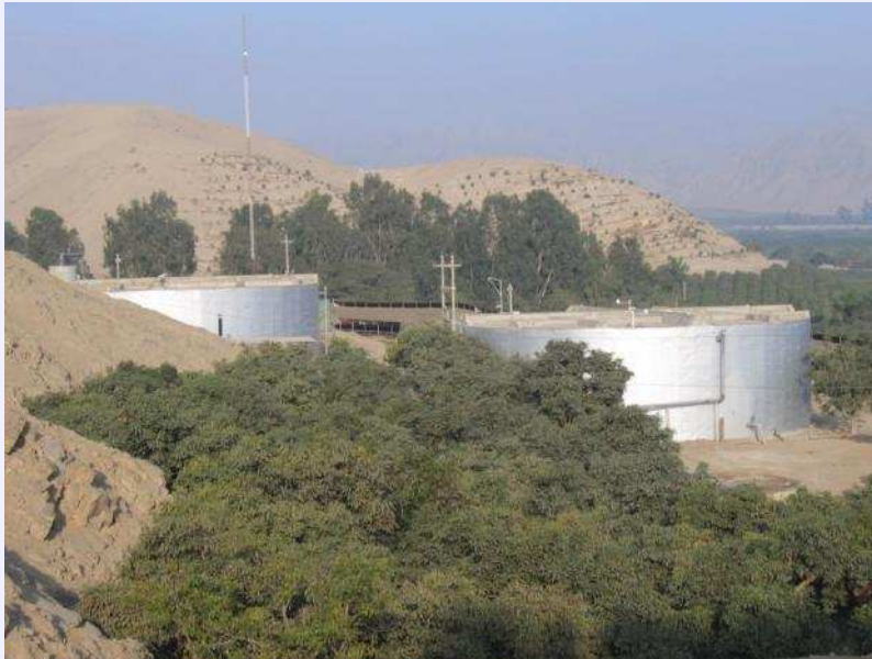
Digester with concrete roof and example of agitator
